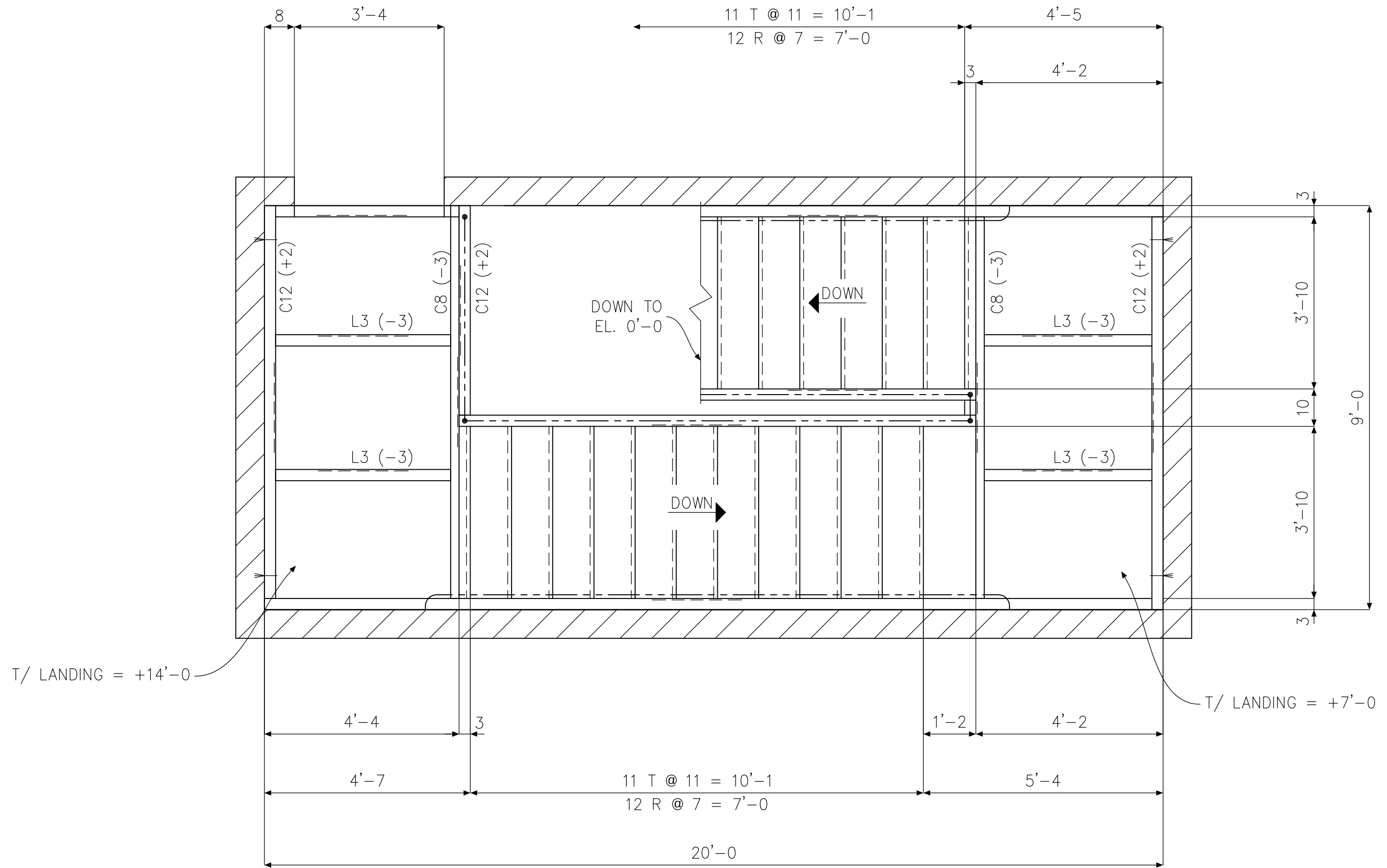
PLAN OF STAIR
